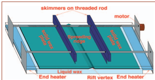
▲ Fig. 2: Schematic diagram of the experimental setup. A rectangular tank of size 114 x 36 x 10 cm 3 is filled with Shell Callista 158 wax which melts at about 72° C. The mechanical properties of micro-crystalline wax are brittle at room temperature and paste-like close to the melting point. No detailed mechanical measurements are performed. The tank is heated from below to (80.0 ± 0.05)°C and cooled from above by a constant flow of air at (12.0 ± 2.0)°C. The weakly turbulent refrigerated air flow is directed vertically downward. Before each run the wax is brought to temperature equilibrium at which a layer of solid wax is present on the surface. Skimmers embedded in the solid wax are attached to a threaded rod that is driven by a micro-stepping motor. A detailed description of this setup has been previously published [11]. The rift is initiated with a straight cut through the wax, perpendicular to the spreading direction. Divergence at this cut causes liquid wax to rise into the rift and solidify. Illumination from below permits us to image the plate thickness at the rift from above using a video camera. As the wax plate thickens it scatters more of the transmitted light and appears darker. In images of wax microplates shown here, spreading is toward the top and bottom of the image and the rift appears as a dark line. The figure is from Ref. [1]
